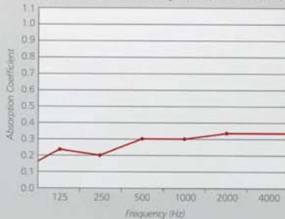
Colinwell Hollow Masonry Block (215mm thick)
