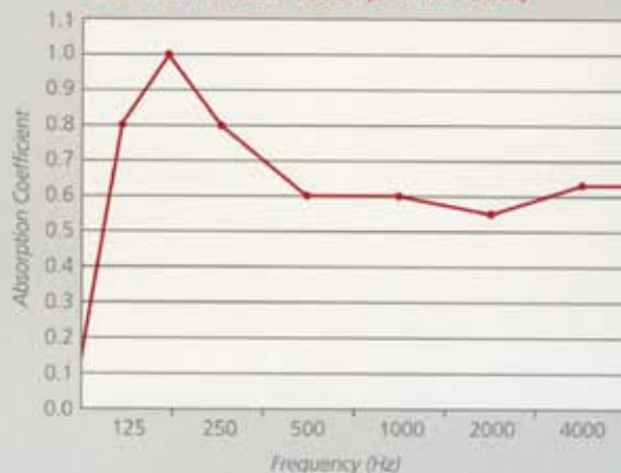
Colinwell Acoustic Block (215mm thick)
